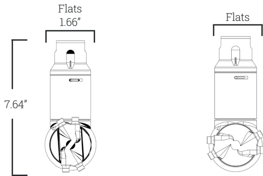
Vertical Nozzle Head Alignment Horizontal Nozzle Head Alignment Clearance Diameter: 3.35" Clearance Diameter: 3.94"
