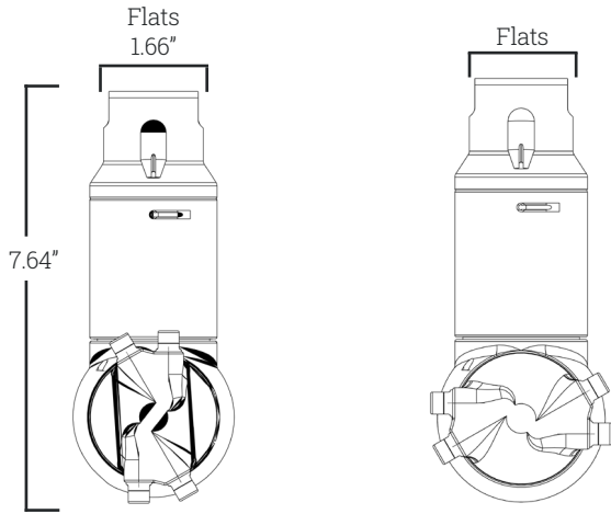
Vertical Nozzle Head Alignment Clearance Diameter: 3.35" Horizontal Nozzle Head Alignment Clearance Diameter: 3.94"
